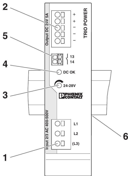
Figure 2 Function elements
